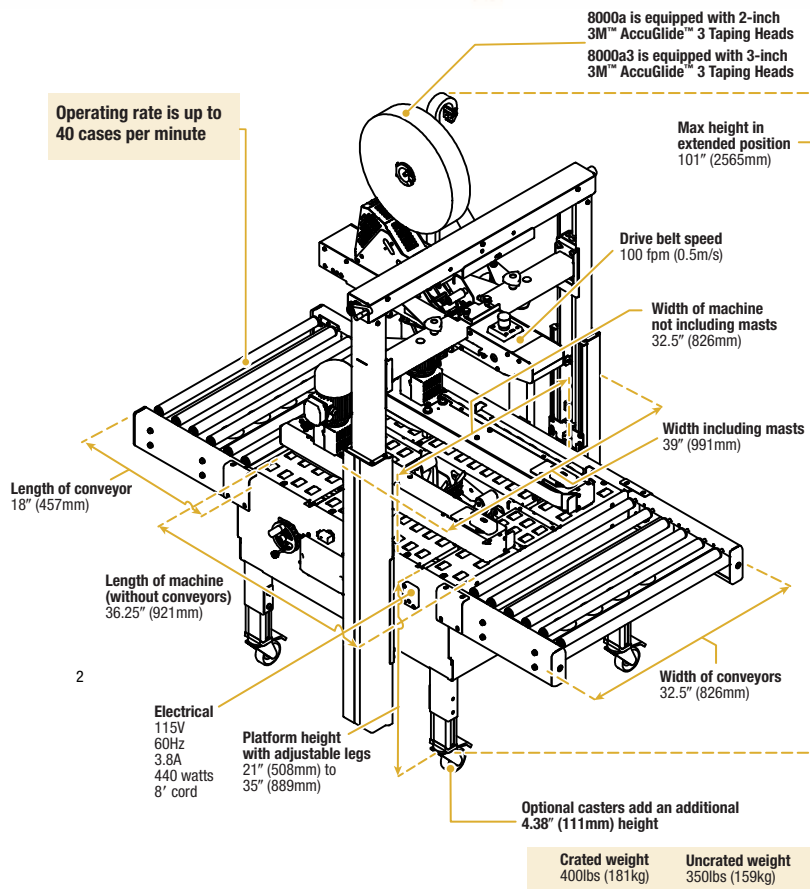
Box Dimensions for 8000a and 8000a3 Machines: Inches (mm)
